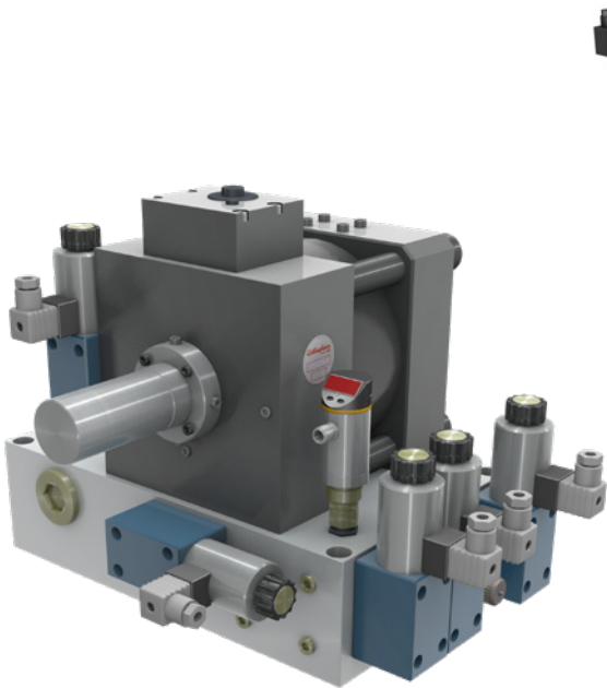
Progressive control units inclusive press safety valves
